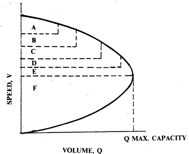
Fig 1. Speed, volume curve showing levels of service
